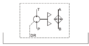
FIGURE NO. 6 HYDRAULIC MOTOR
