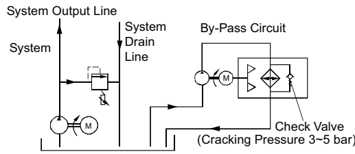
FIGURE NO. 5 By-Pass Circuit
